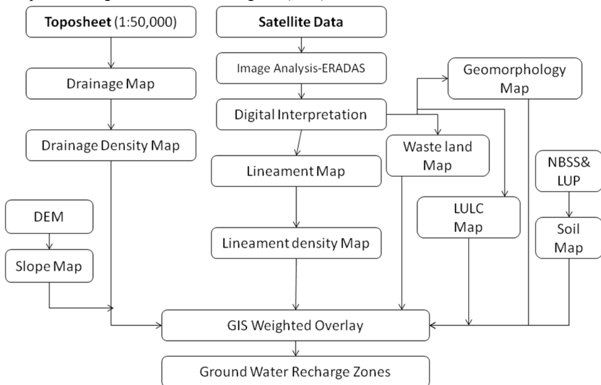
Fig.3.1. Flow chart for identifying groundwater recharge zones
